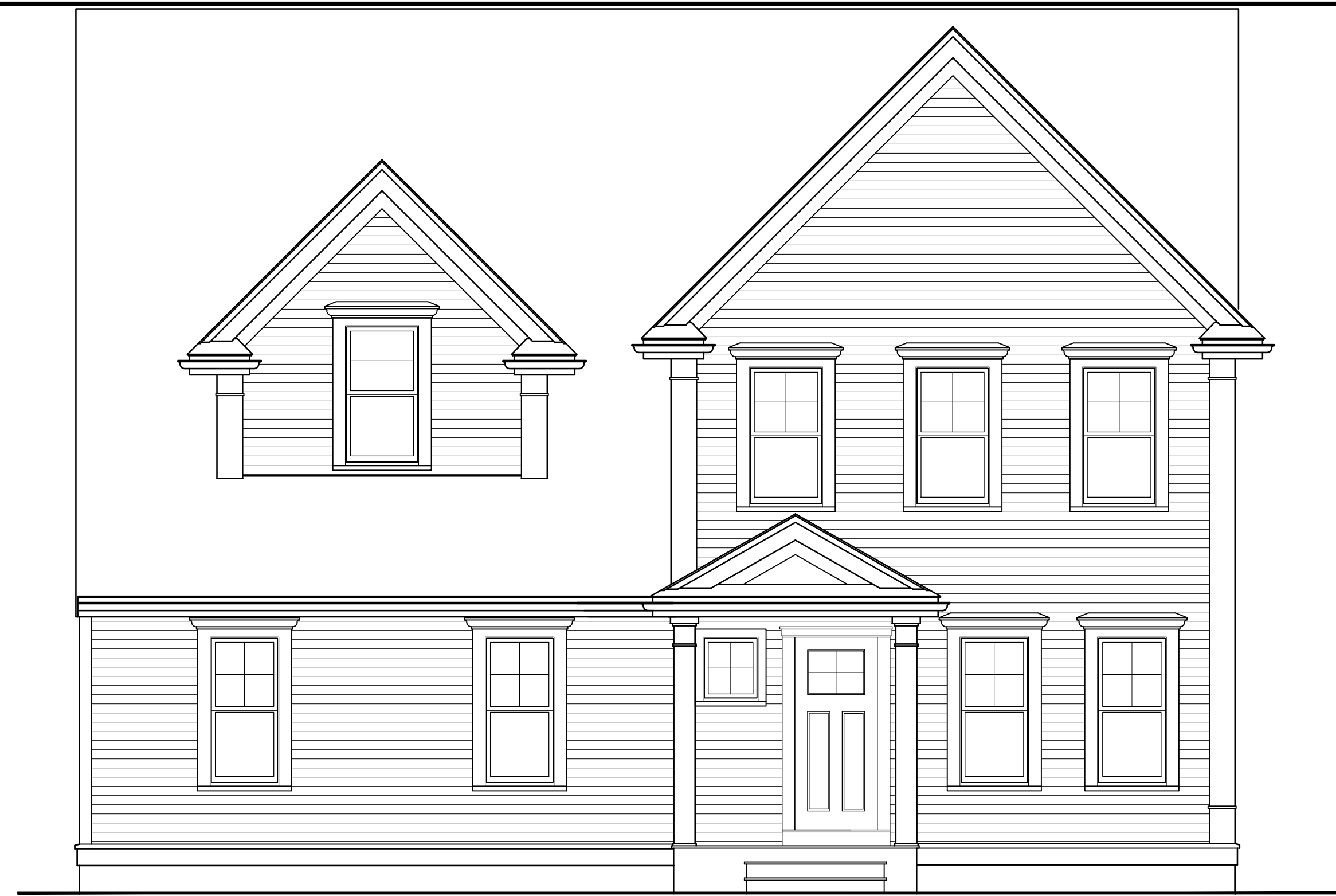
FRONT ELEVATION A.1
