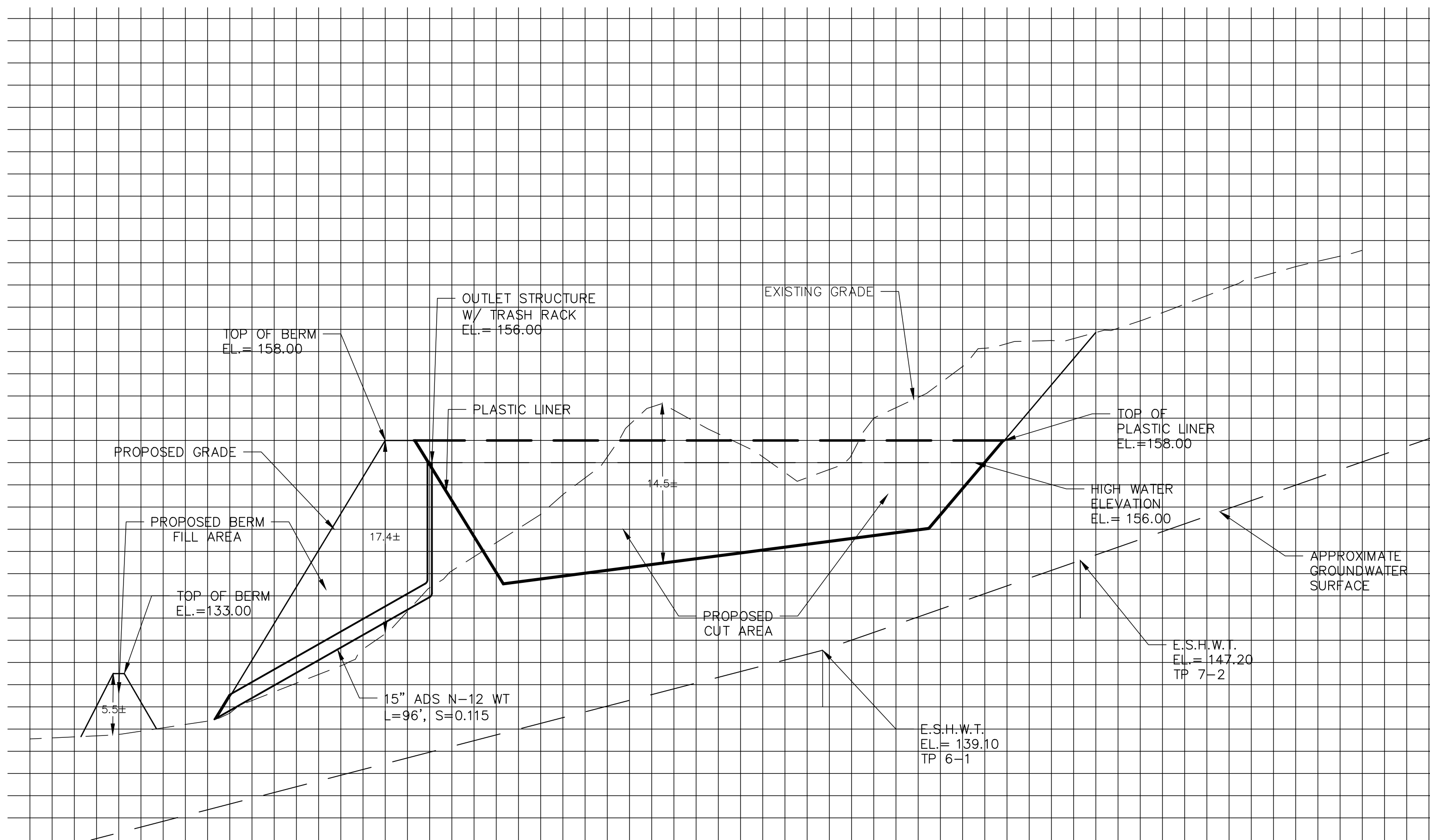
OUTLET STRUCTURE PROFILE (SECTION 1)
