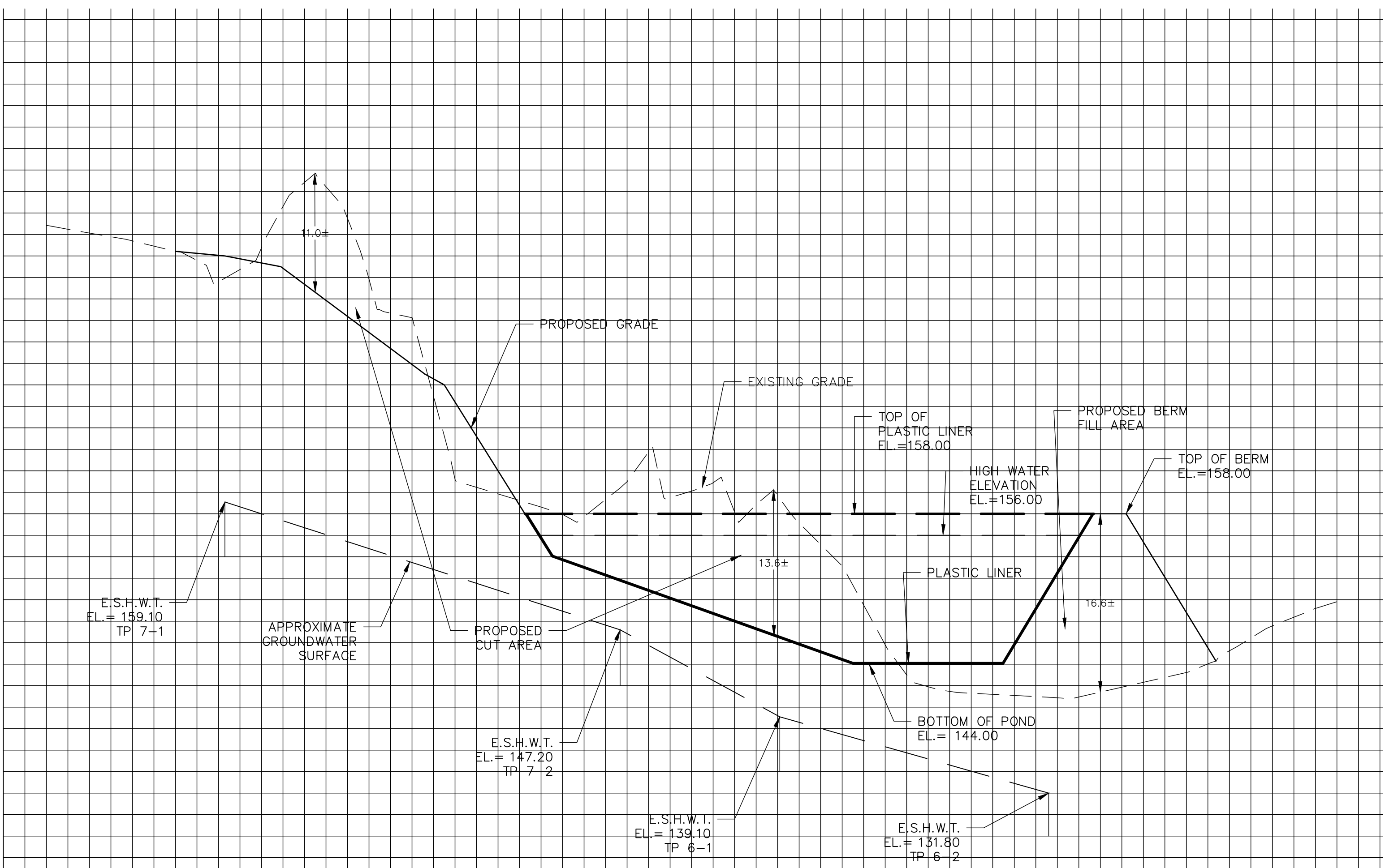
BOTTOM OF POND PROFILE (SECTION 2)
